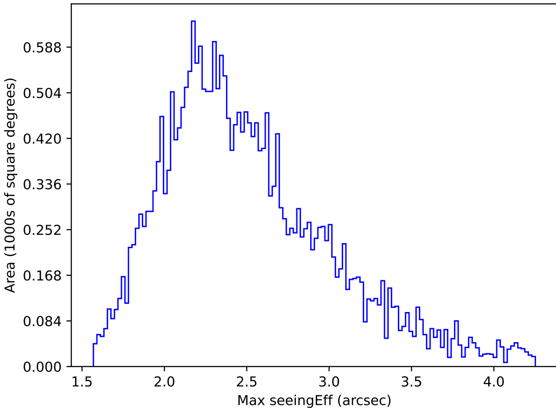
noroll_v3.4_10yrs All sky r band: Max seeingEff
