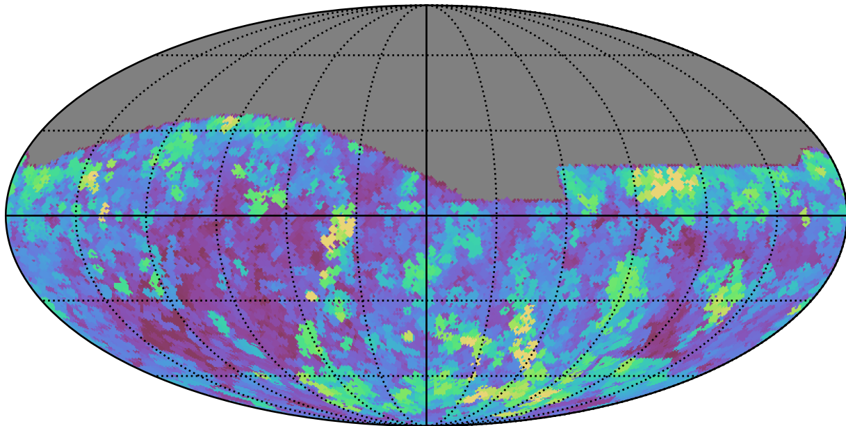
noroll_v3.4_10yrs All sky g band: Max seeingEff
