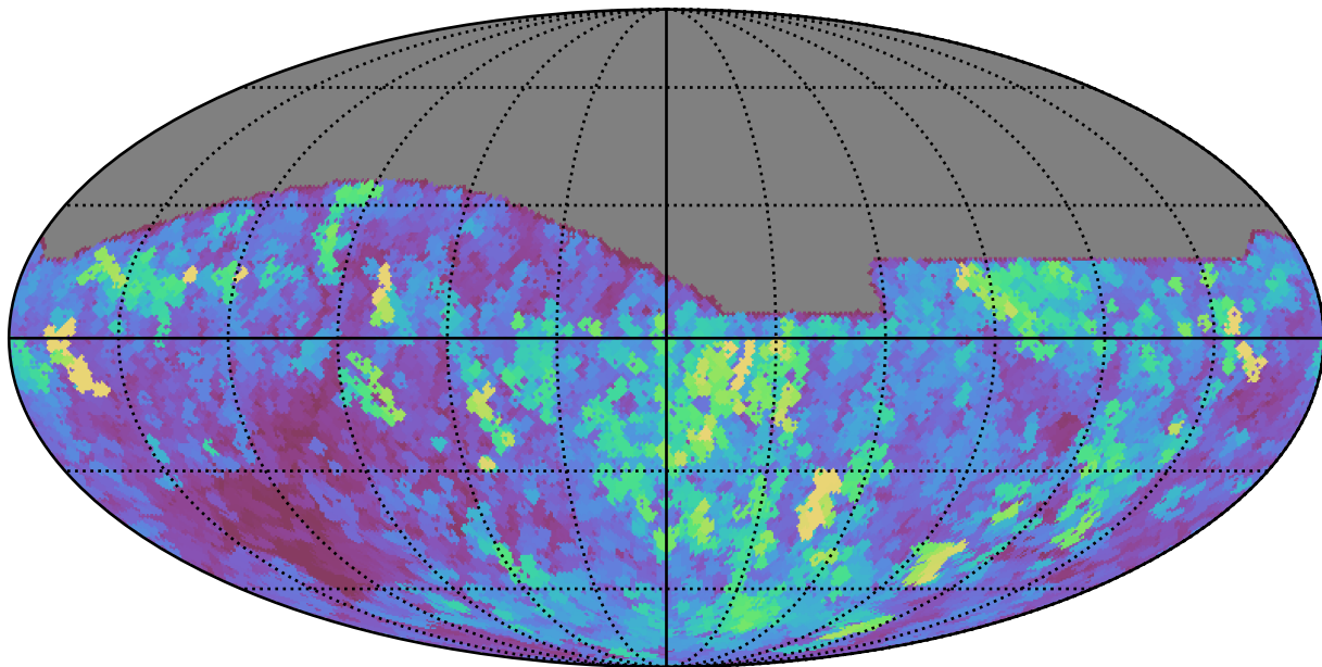
noroll_v3.4_10yrs All sky all bands: Max seeingEff
