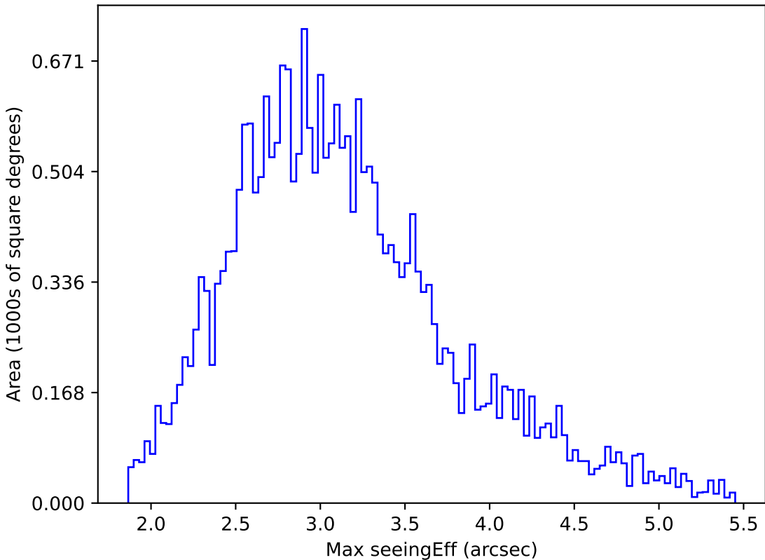
noroll_v3.4_10yrs All sky all bands: Max seeingEff
