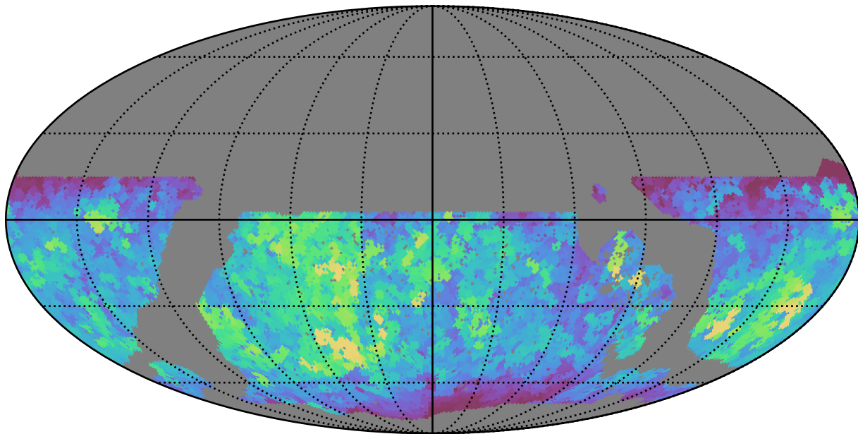
noroll_v3.4_10yrs WFD r band: Max saturation_mag
