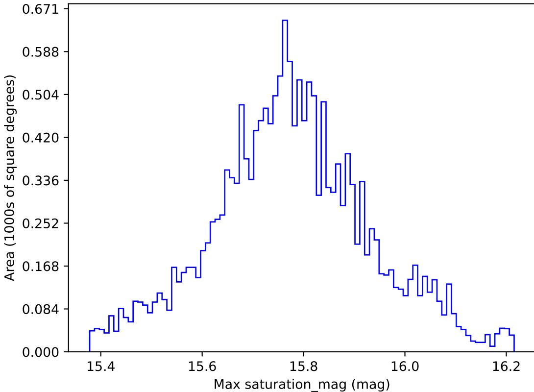
noroll_v3.4_10yrs WFD r band: Max saturation_mag
