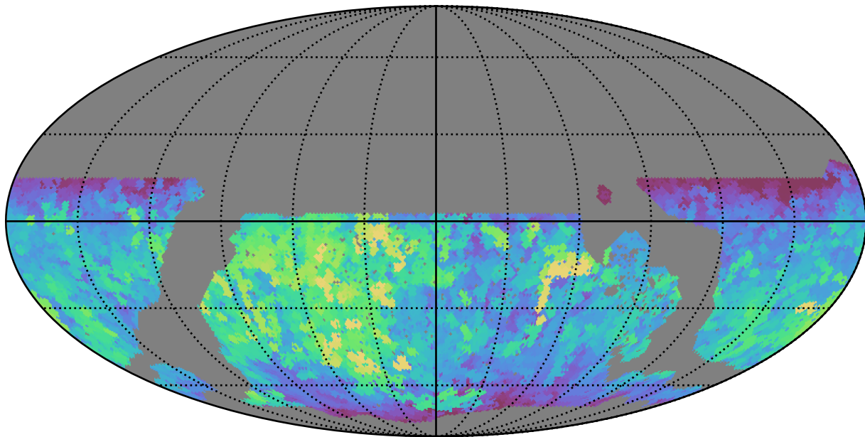
noroll_v3.4_10yrs WFD i band: Max saturation_mag
