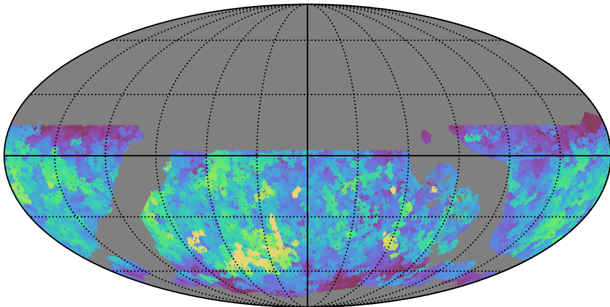
noroll_v3.4_10yrs WFD g band: Max saturation_mag
