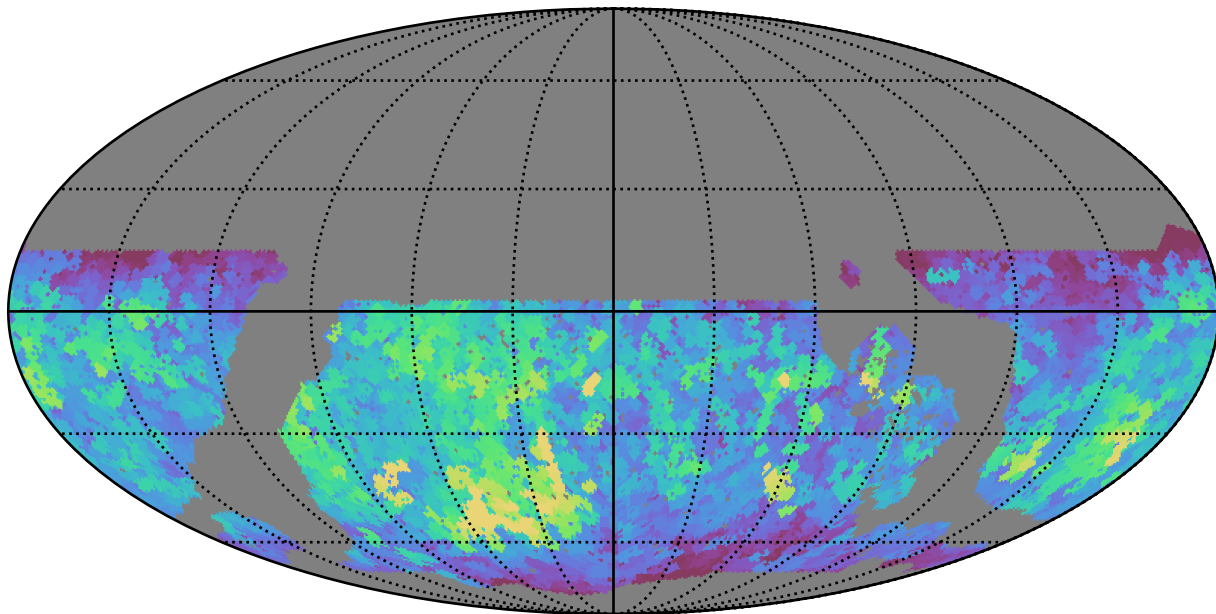
noroll_v3.4_10yrs WFD all bands: Max saturation_mag
