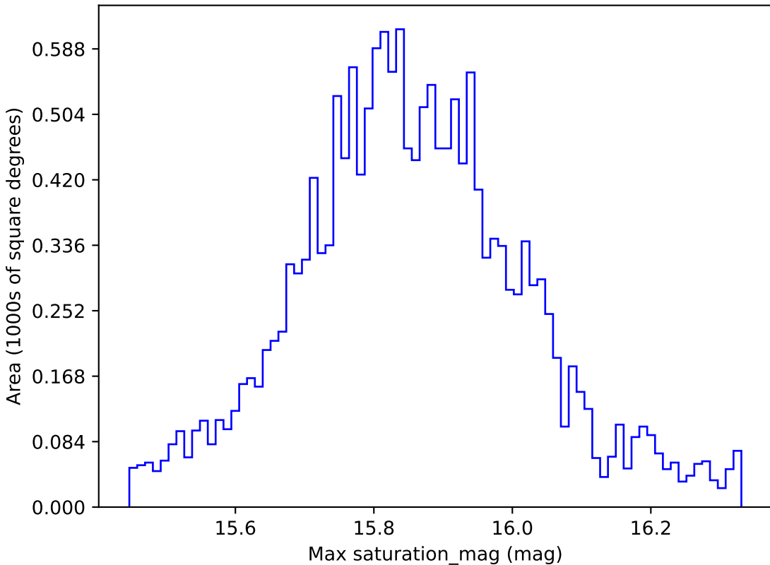
noroll_v3.4_10yrs WFD all bands: Max saturation_mag
