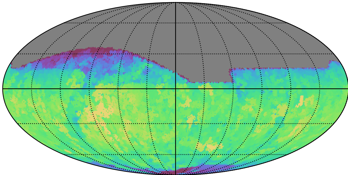
noroll_v3.4_10yrs All sky z band: Max saturation_mag
