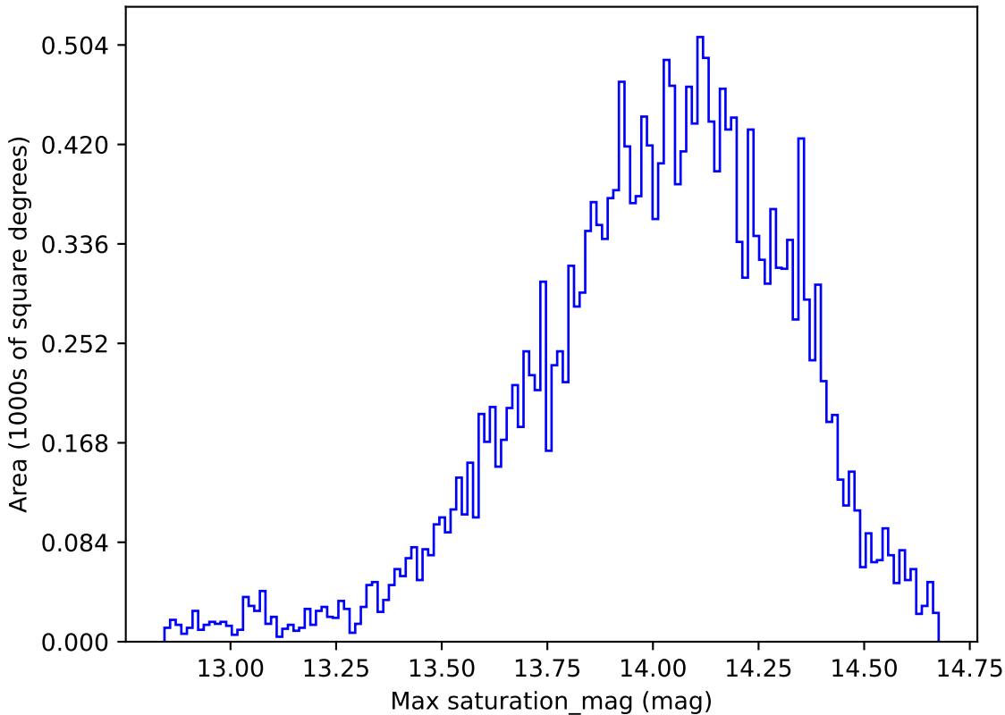
noroll_v3.4_10yrs All sky u band: Max saturation_mag
