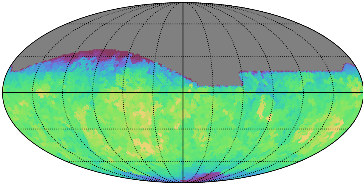
noroll_v3.4_10yrs All sky r band: Max saturation_mag
