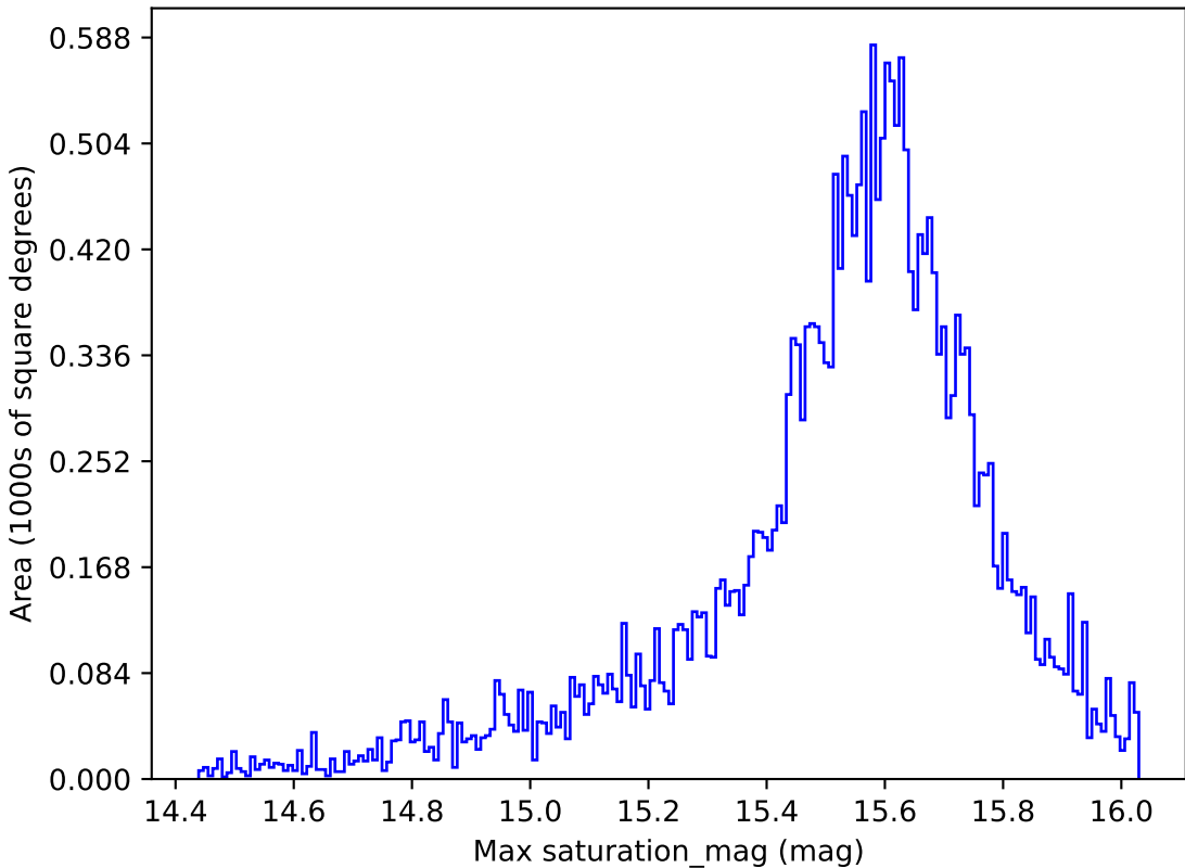
noroll_v3.4_10yrs All sky i band: Max saturation_mag
