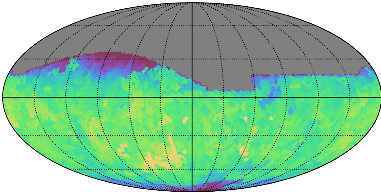
noroll_v3.4_10yrs All sky g band: Max saturation_mag
