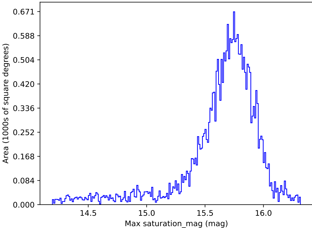
noroll_v3.4_10yrs All sky g band: Max saturation_mag
