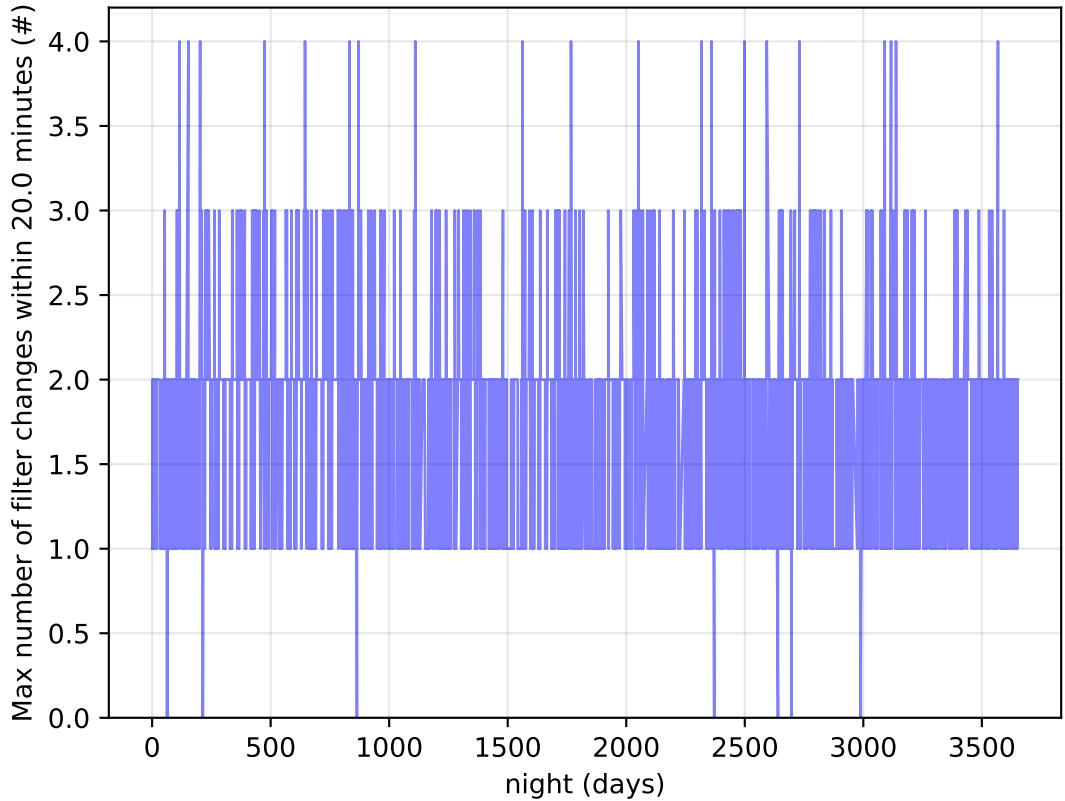
noroll_v3.4_10yrs Per Night: Max number of filter changes within 20.0 minutes
