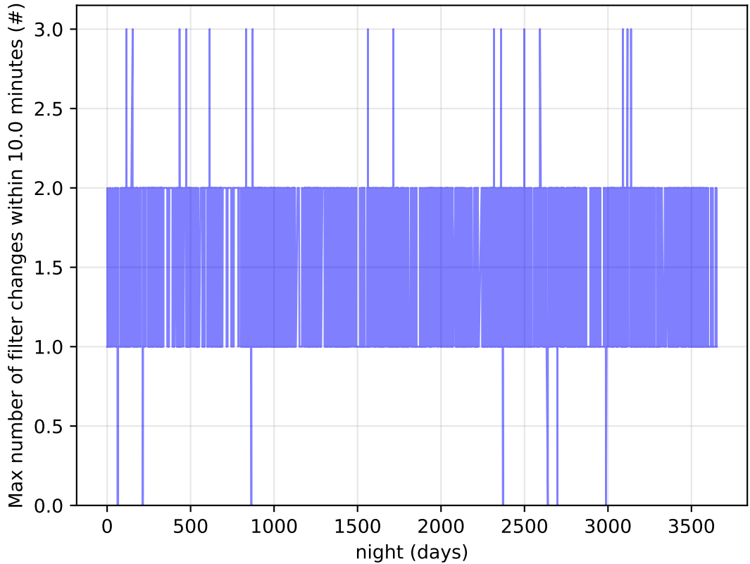
noroll_v3.4_10yrs Per Night: Max number of filter changes within 10.0 minutes
