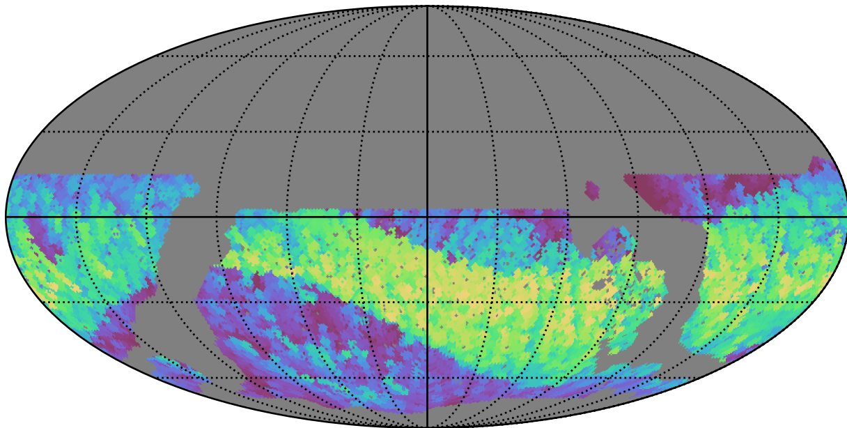
noroll_v3.4_10yrs WFD z band: Max normairmass
