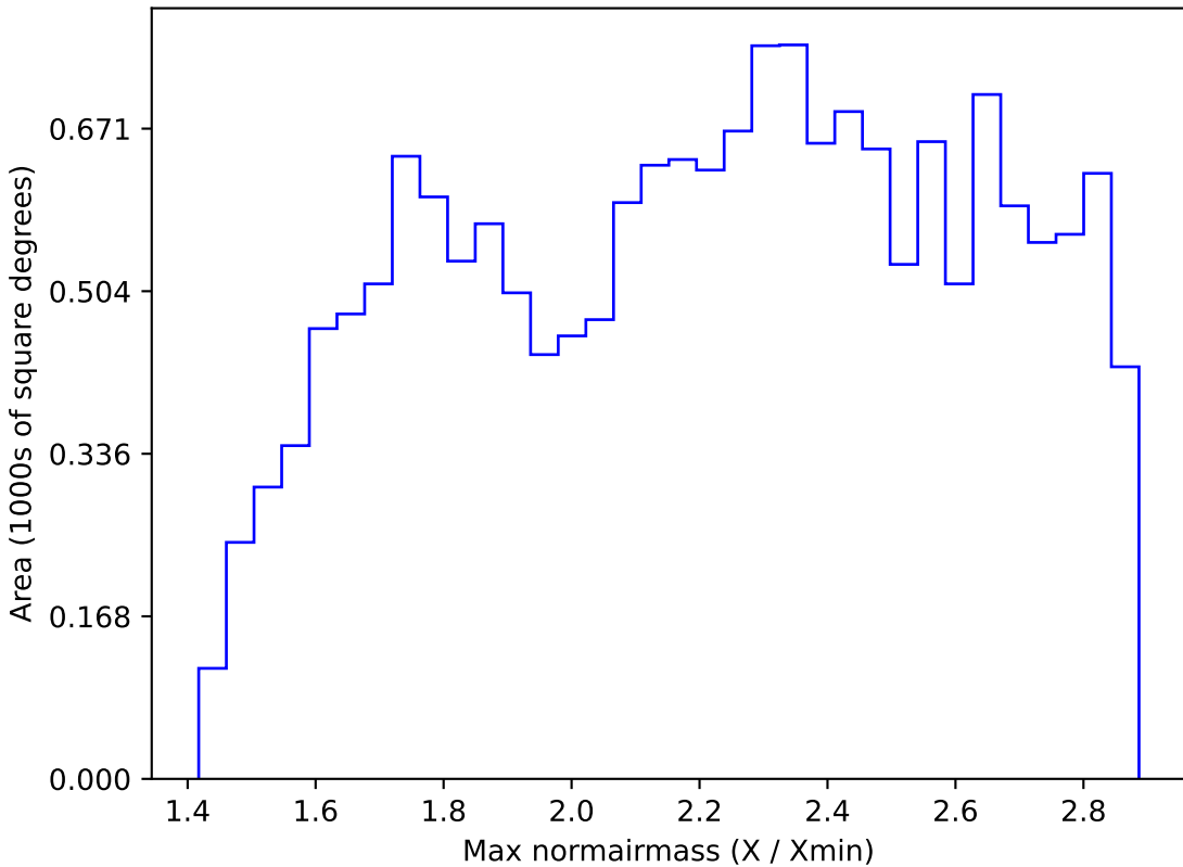
noroll_v3.4_10yrs WFD z band: Max normairmass
