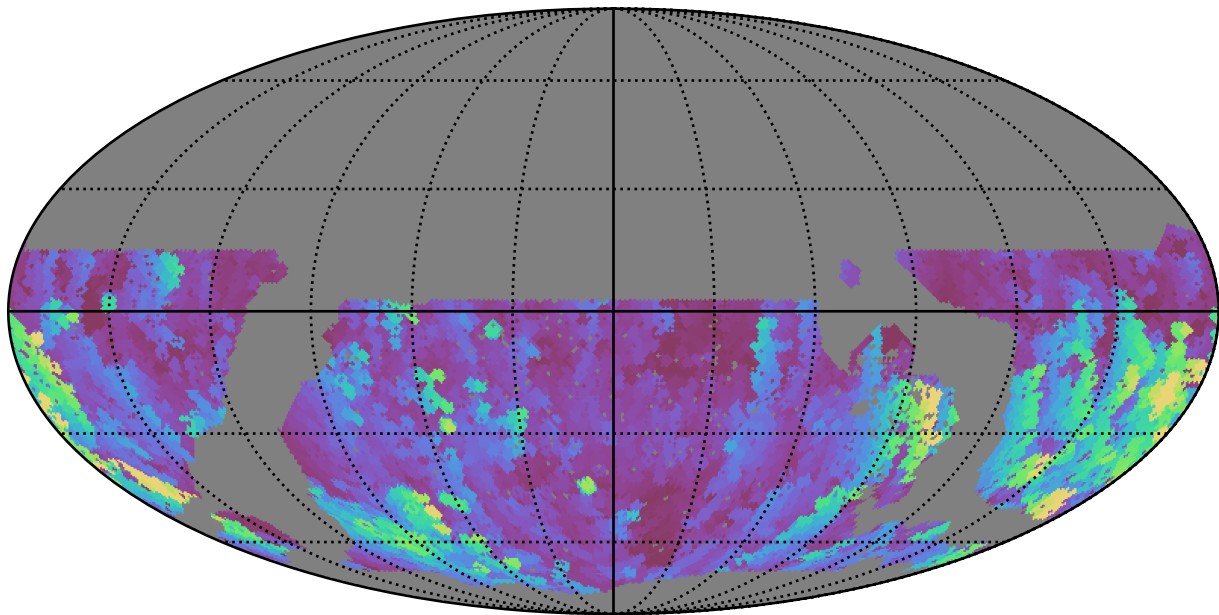
noroll_v3.4_10yrs WFD u band: Max normairmass
