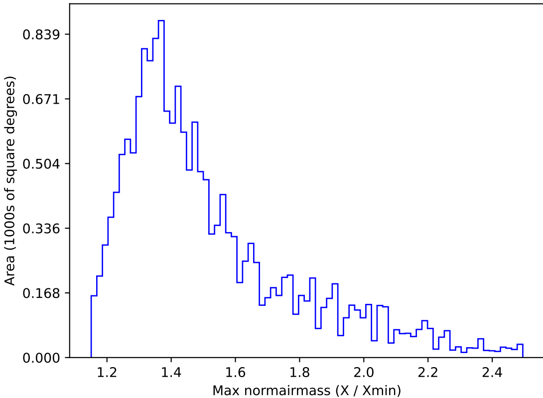
noroll_v3.4_10yrs WFD u band: Max normairmass
