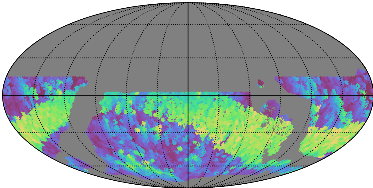
noroll_v3.4_10yrs WFD r band: Max normairmass
