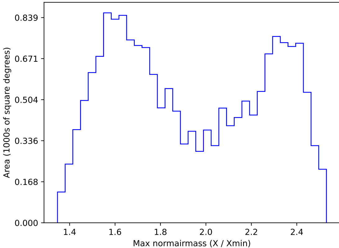
noroll_v3.4_10yrs WFD r band: Max normairmass
