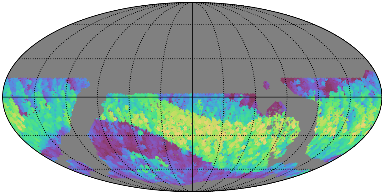
noroll_v3.4_10yrs WFD i band: Max normairmass
