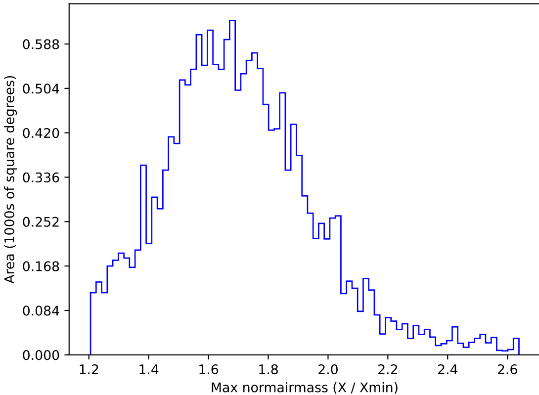
noroll_v3.4_10yrs WFD g band: Max normairmass
