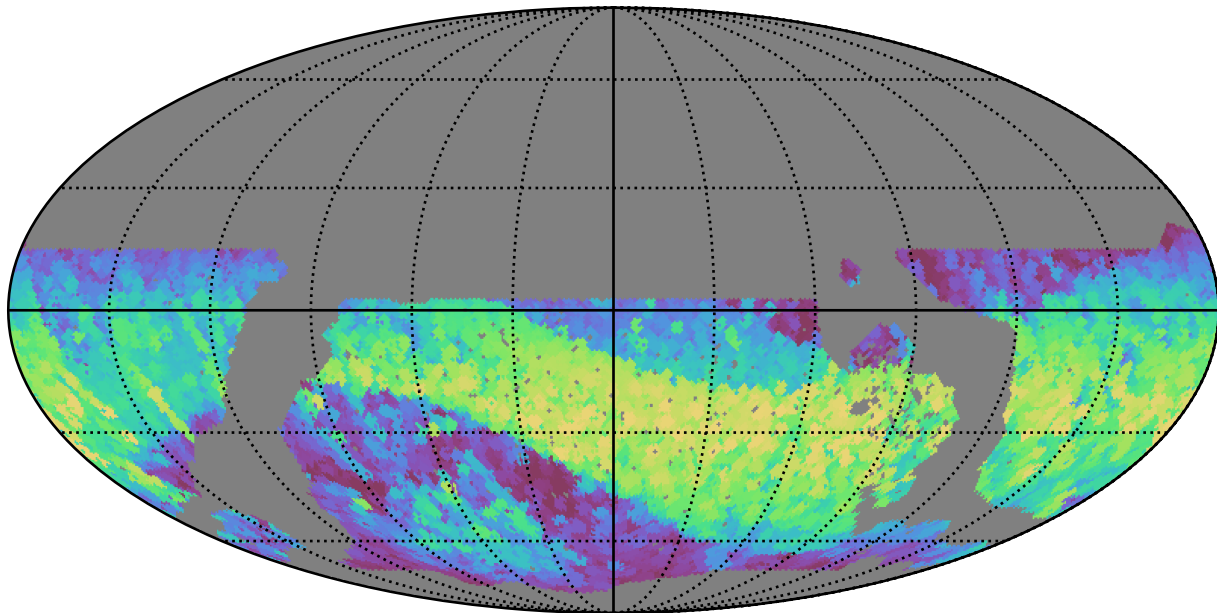
noroll_v3.4_10yrs WFD all bands: Max normairmass
