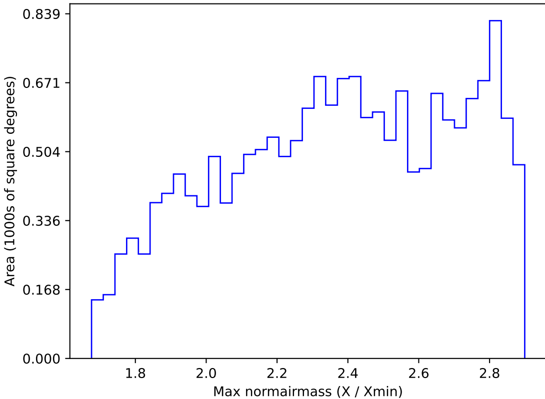
noroll_v3.4_10yrs WFD all bands: Max normairmass
