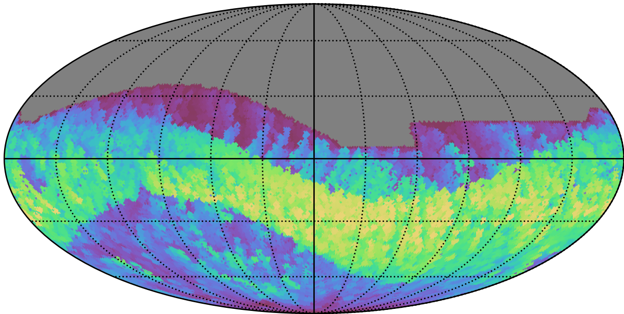
noroll_v3.4_10yrs All sky z band: Max normairmass
