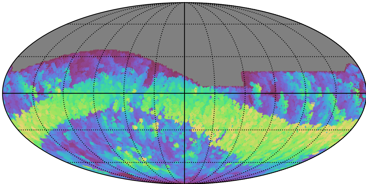
noroll_v3.4_10yrs All sky r band: Max normairmass
