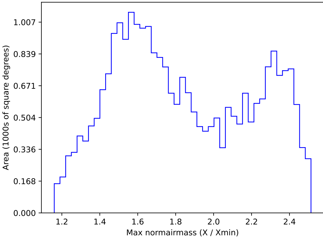
noroll_v3.4_10yrs All sky r band: Max normairmass
