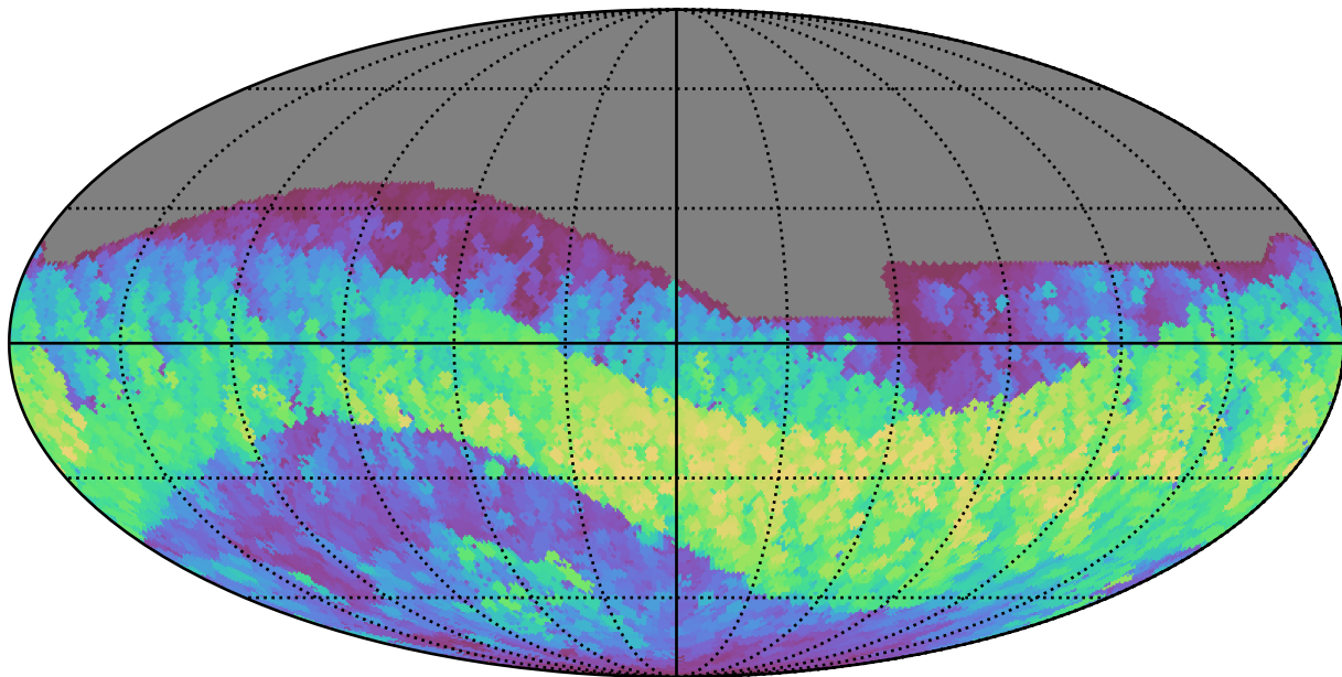
noroll_v3.4_10yrs All sky i band: Max normairmass
