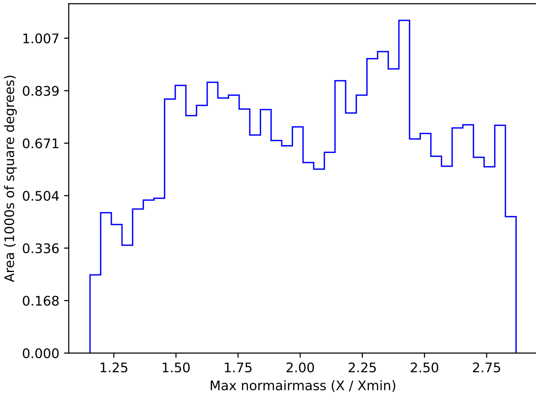
noroll_v3.4_10yrs All sky i band: Max normairmass
