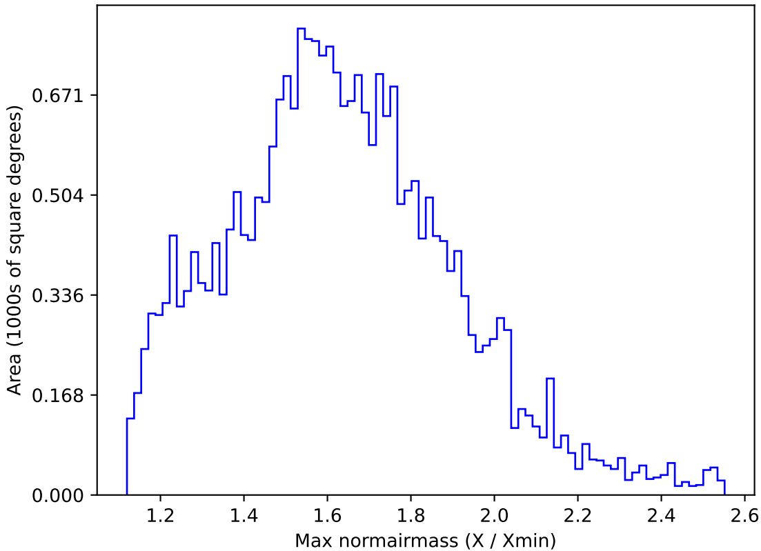
noroll_v3.4_10yrs All sky g band: Max normairmass
