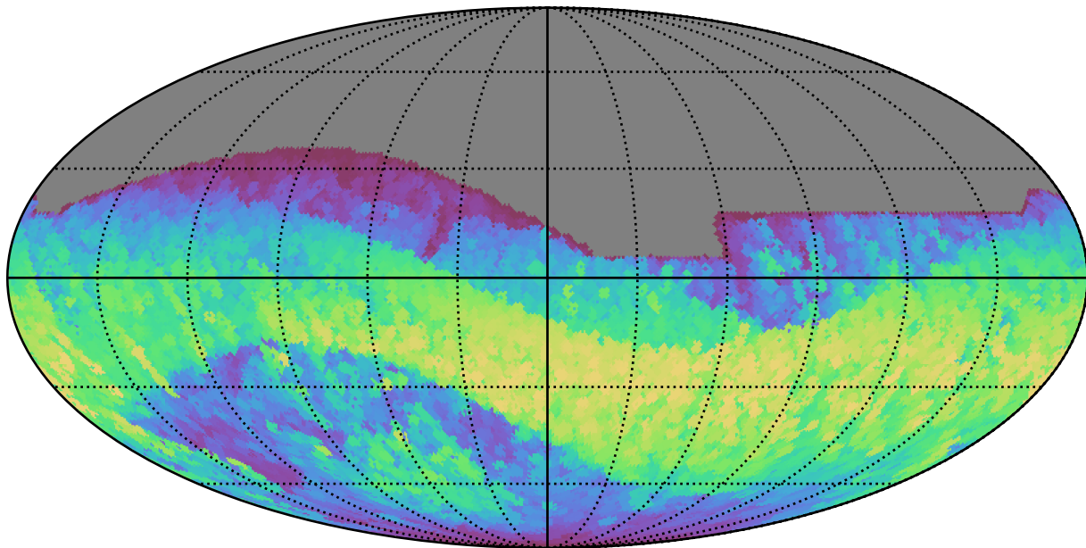
noroll_v3.4_10yrs All sky all bands: Max normairmass
