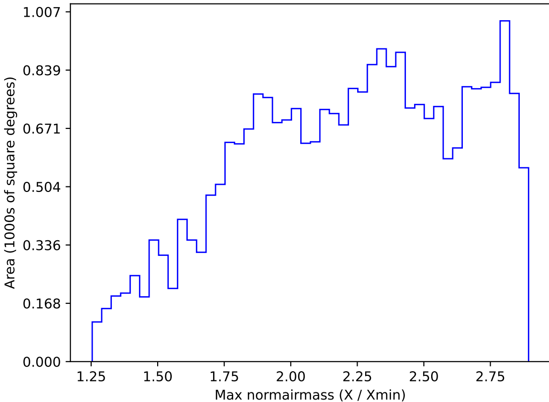
noroll_v3.4_10yrs All sky all bands: Max normairmass
