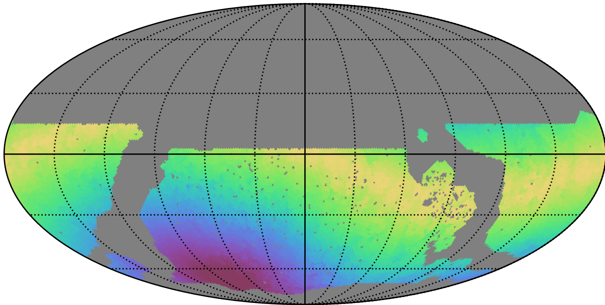
noroll_v3.4_10yrs WFD z band: Max moonDistance
