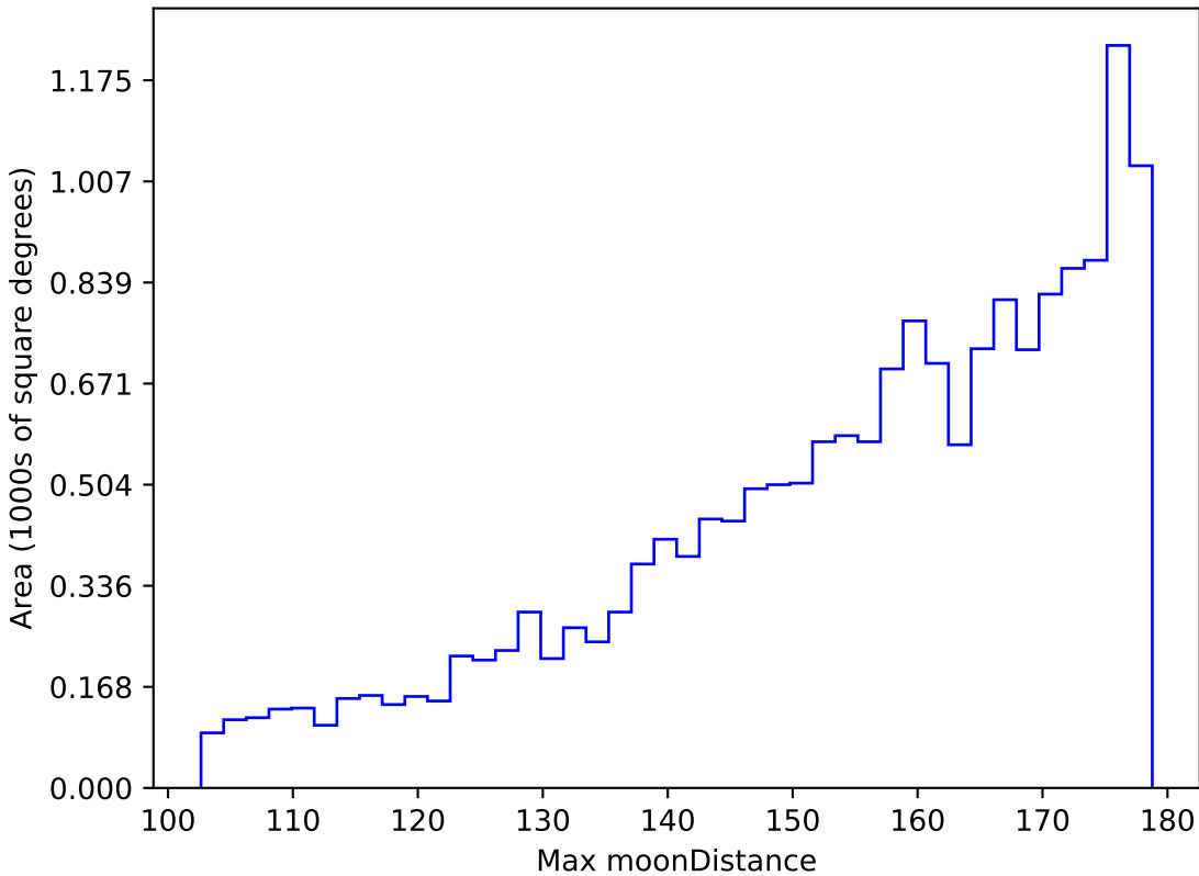
noroll_v3.4_10yrs WFD z band: Max moonDistance
