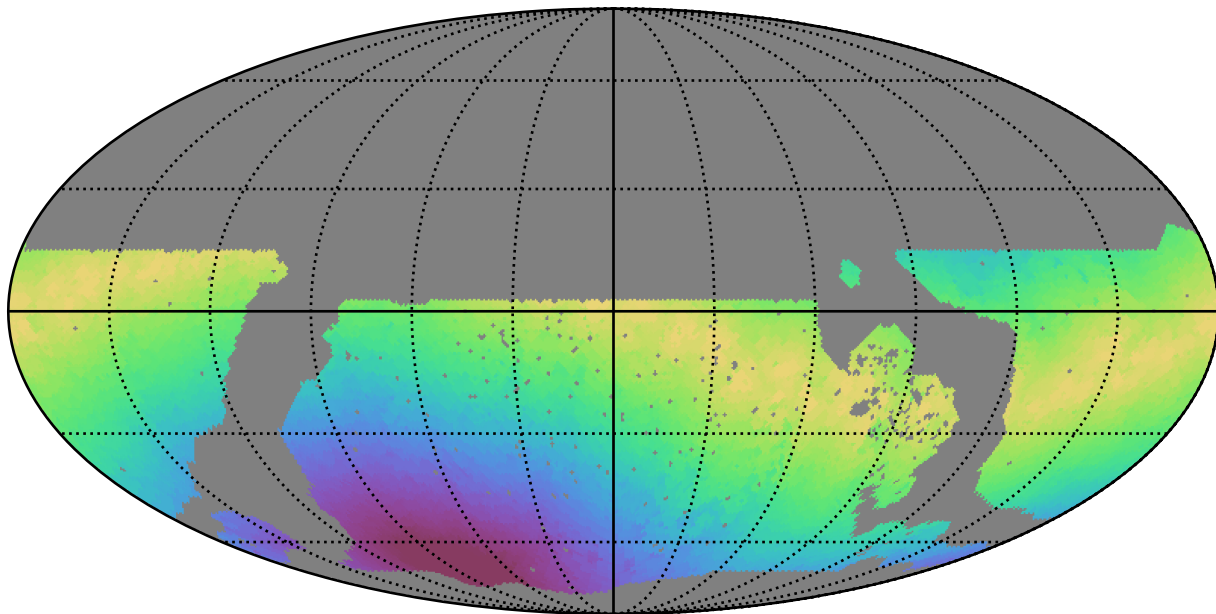
noroll_v3.4_10yrs WFD u band: Max moonDistance
