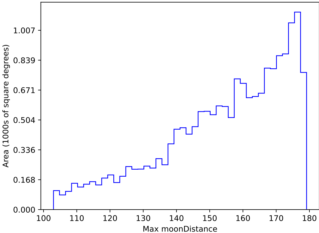
noroll_v3.4_10yrs WFD u band: Max moonDistance
