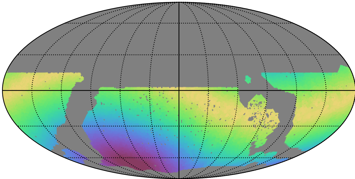
noroll_v3.4_10yrs WFD r band: Max moonDistance
