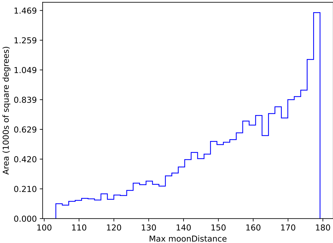
noroll_v3.4_10yrs WFD i band: Max moonDistance
