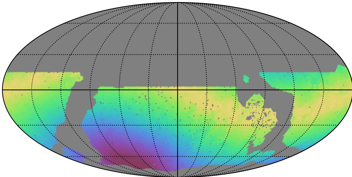
noroll_v3.4_10yrs WFD g band: Max moonDistance
