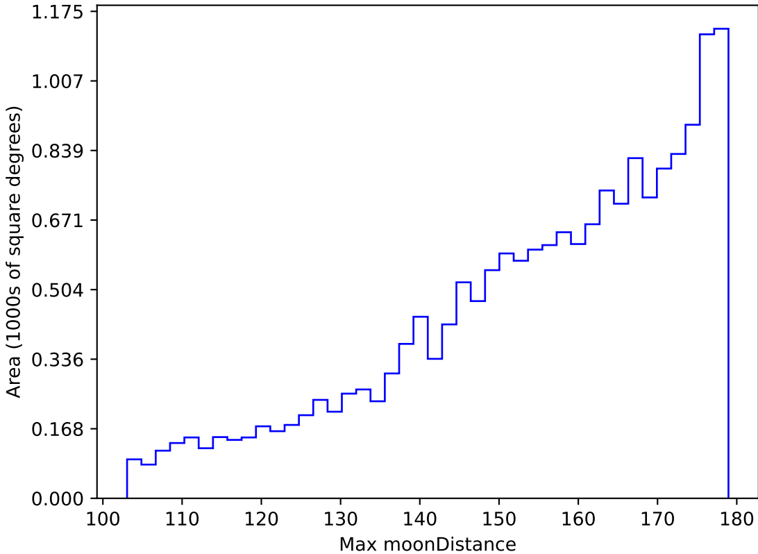
noroll_v3.4_10yrs WFD g band: Max moonDistance
