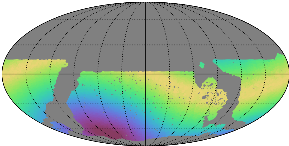
noroll_v3.4_10yrs WFD all bands: Max moonDistance
