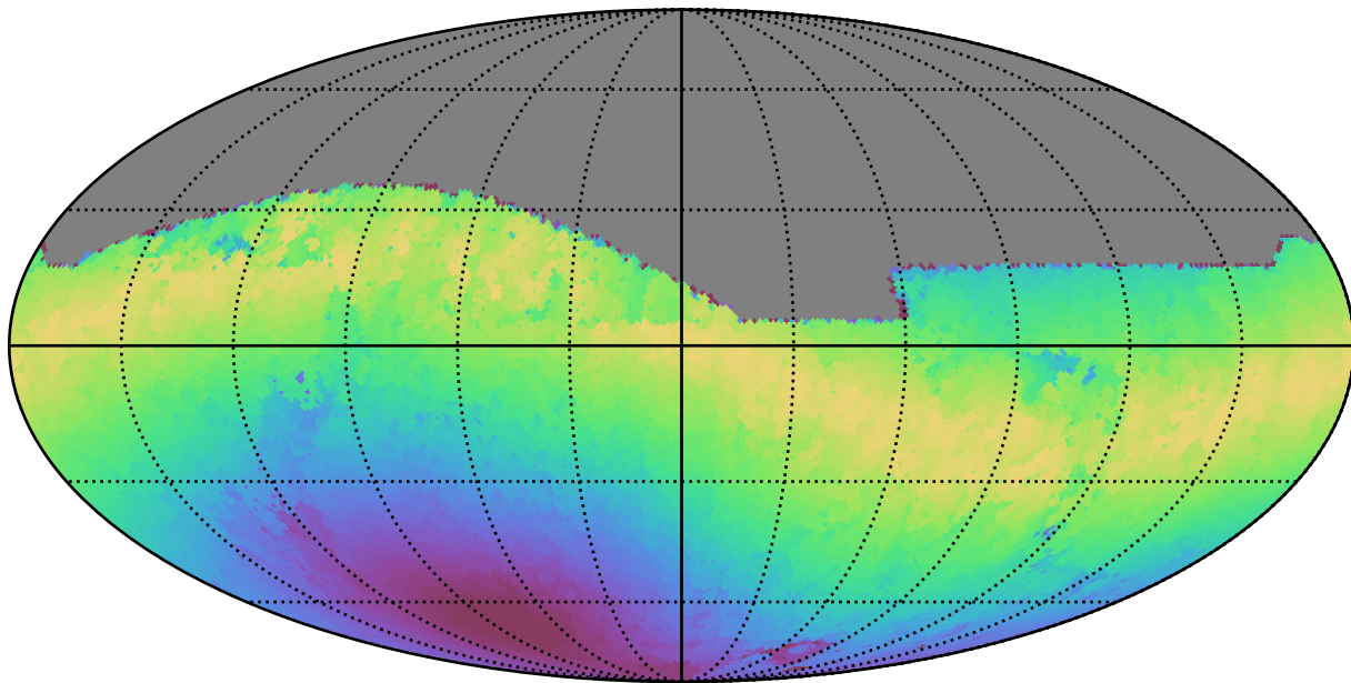
noroll_v3.4_10yrs All sky z band: Max moonDistance
