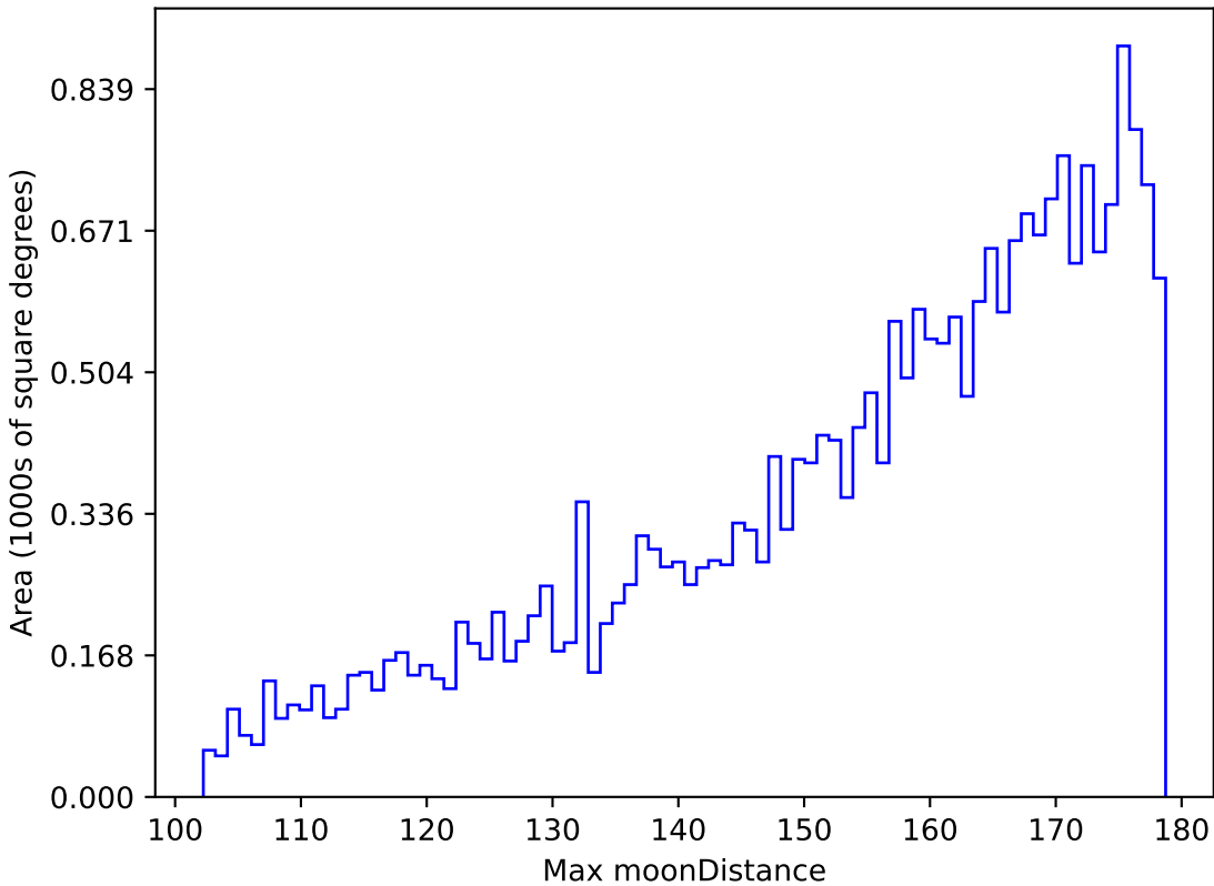
noroll_v3.4_10yrs All sky z band: Max moonDistance
