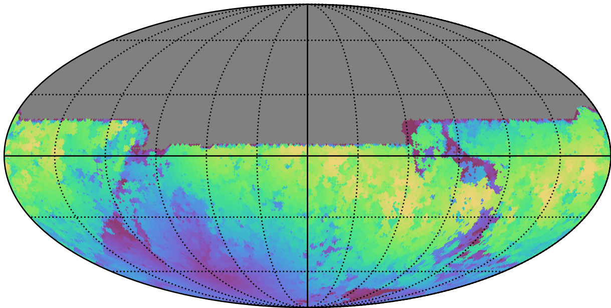
noroll_v3.4_10yrs All sky y band: Max moonDistance
