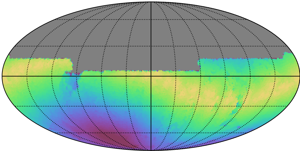
noroll_v3.4_10yrs All sky u band: Max moonDistance
