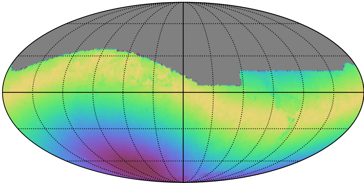
noroll_v3.4_10yrs All sky r band: Max moonDistance
